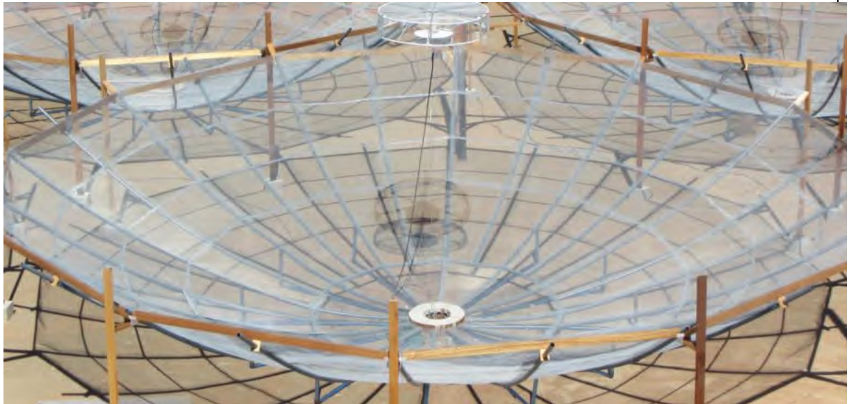
Figure 1: One of the HERA prototype dishes
