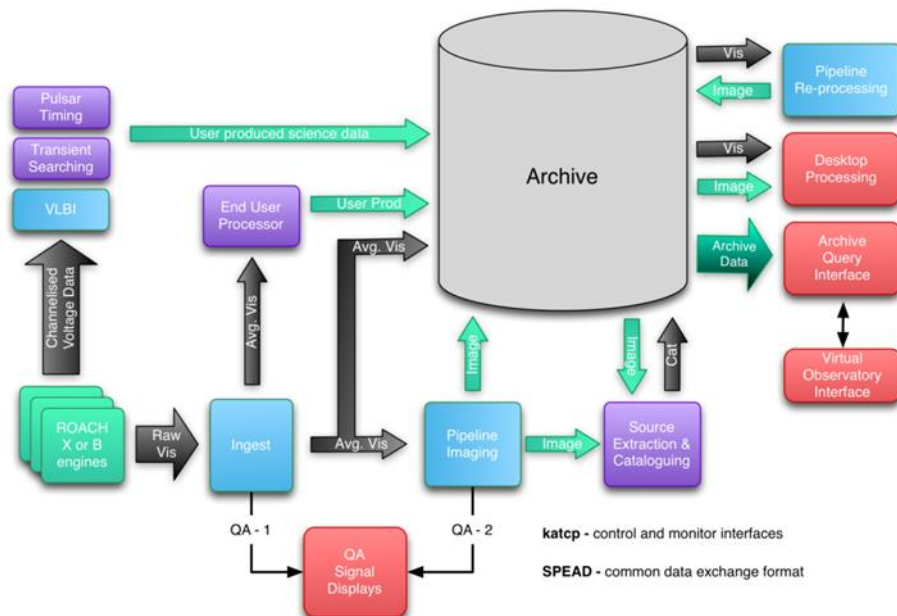
Figure 1: Science Data Processor core components and data channels
