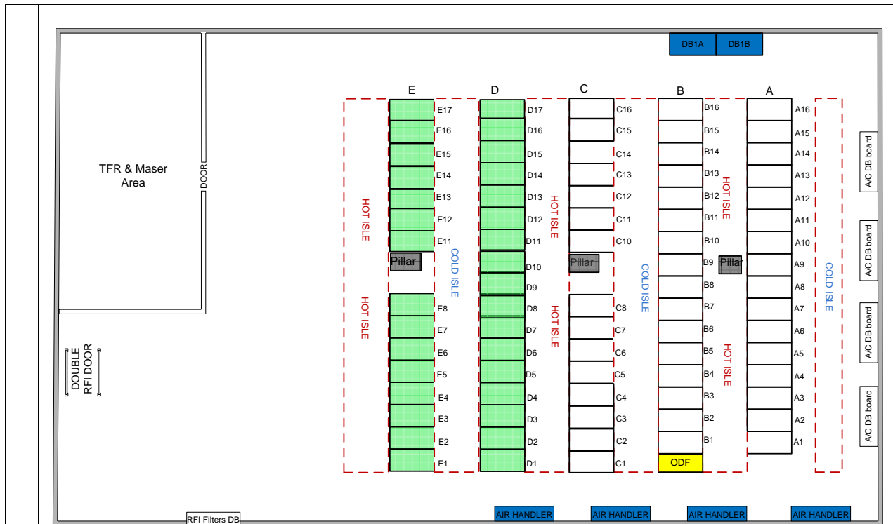
Figure 1: Rack Layout
